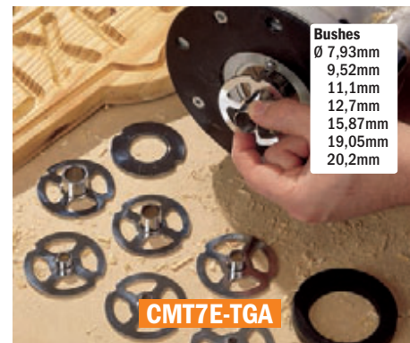
CMT7E-TGA Template guide kit includes 7 guide bushes, a guide plate, and alignment bush, and spacers. It could be used with CMT7E and CMT8E routers.
